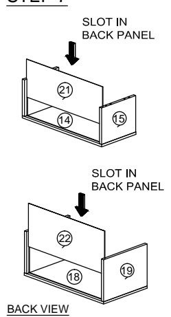
BACK VIEW
